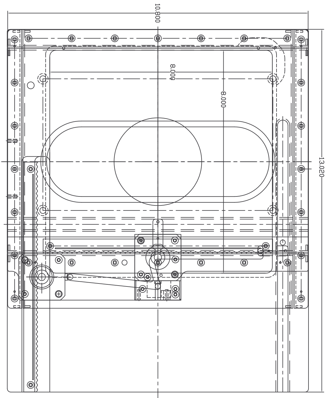
BOTTOM VIEW
